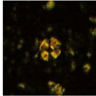
Tegulalithus tesselatus
