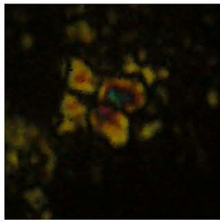
Tetralithus cassianus
