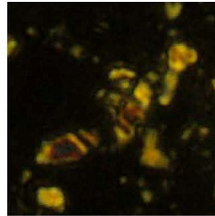
Corollithion signum
