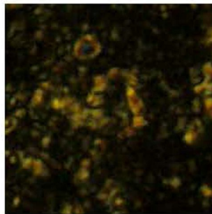
Nannoconus wassallii
