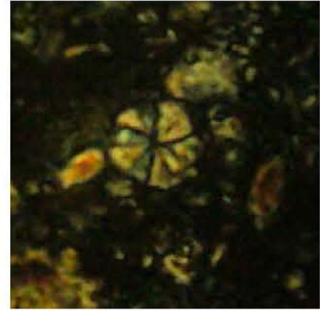
Radiolitus planus
