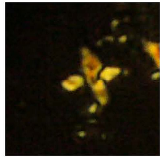
Tetralithus cassianus
