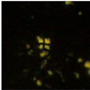
Tetralithus cassianus
