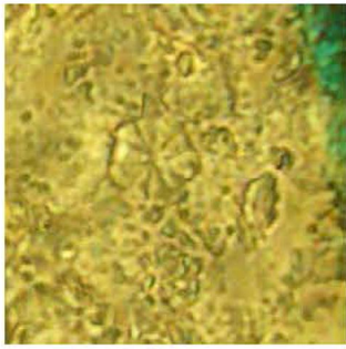
Radiolitus planus
