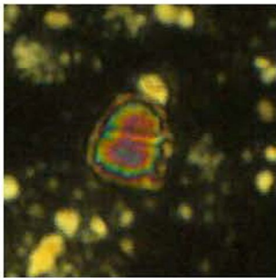
Nannoconus circularis
