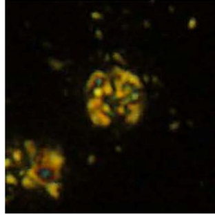
Polycostella beckmanii
