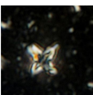
Micula decussata Image # Abtalkh8 (K)
