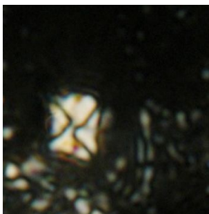
Micula. swastica Image # Abtalkh6 (K)
