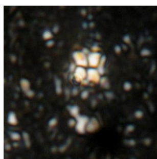
Quadrum gothicus Image # Abderaz2 (K)
