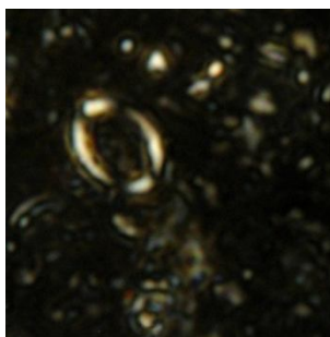
Cribrosphaerella ehrenbergii Image # Abtalkh8 (M)
