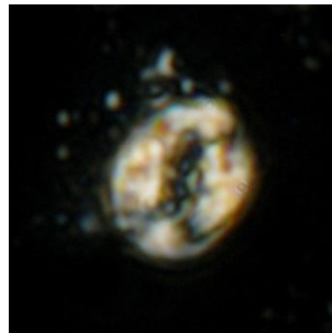
Aspidolithus parvus constrictus Image # Abtalkh6 (M)
