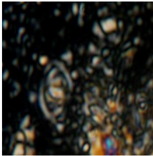
Zeugrhabdotus spiralis Image # Abtalkh9 (K)
