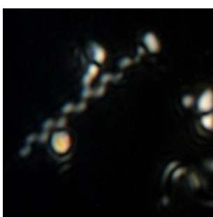
Microrhabdulus decoratus Image # Abderaz 4 (M)
