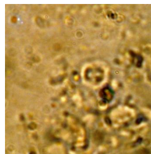
Prediscosphaera spinosa Image # Abtalkh10 (K)
