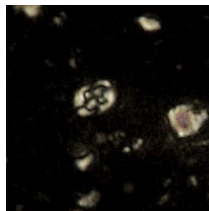
Staurolithites ellipticus Image # Abtalkh6 (K)
