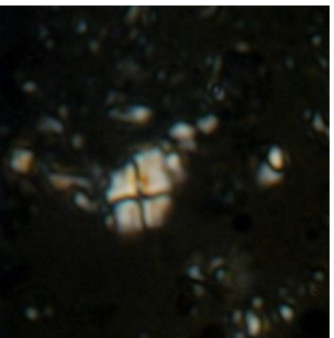
Calculites ovalis Image # Abderaz 2 (K)
