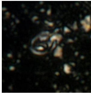
Zeugrhabdotus scutula Image # Abtalkh7 (K)
