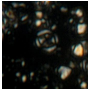
Arkhangelskiella specillata Image # Abtalkh8 (K)
