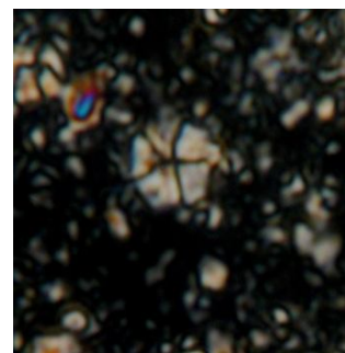
Braarudosphaera africana Image # Abtalkh 9 (K)
