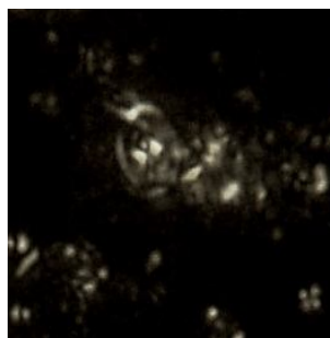
Reinhardtites anthophorus Image # Abtalkh9 (K)
