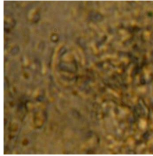
Zeugrhabdotus spiralis Image # Abtalkh 9 (K)
