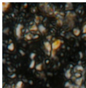
Ceratolithoides aculeus Image # Abderaz1 (M)
