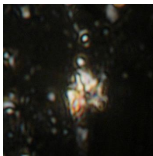
Bukryaster hayi Image # Abtalkh8 (K)
