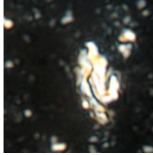
Lucianorhabdus cayeuxii Image # Abtalkh5 (M)
