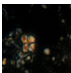
Quadrum garneri Image # Abderaz1 (M)
