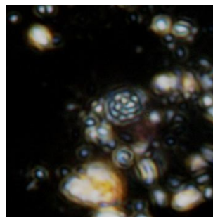
Prediscosphaera spinosa Image # Abtalkh10 (K)
