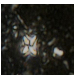
Uniplanarius sissinghii Image # Abderaz3 (K)
