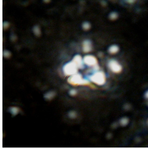
Eprolithus moratus Image # Abderaz3(K)
