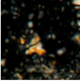
Lucianorhabdus maleformis Image # Abtalkh7 (K)
