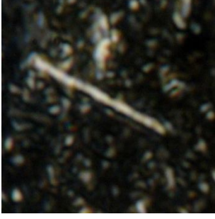
Lithraphidites carniolensis Image # Abderaz3 (M)
